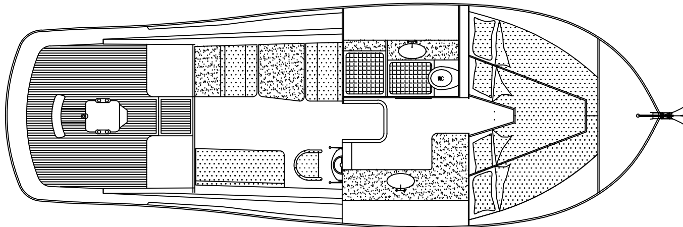
PLAN BELOW DECK
